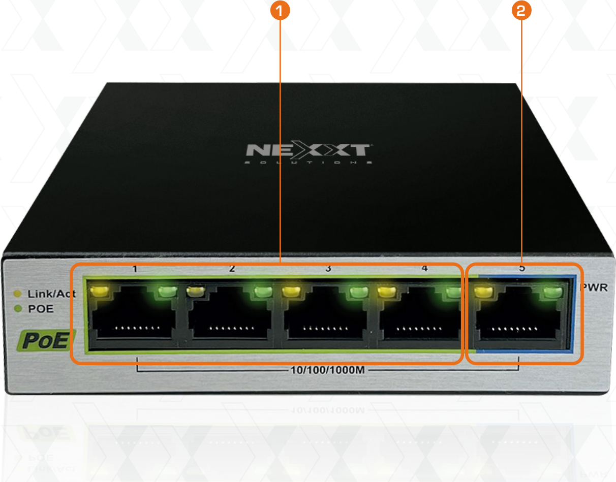
Front View
